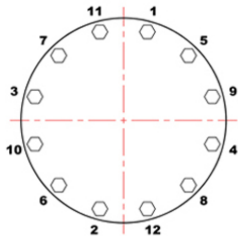
12 BOLT FLANGE not to scale
