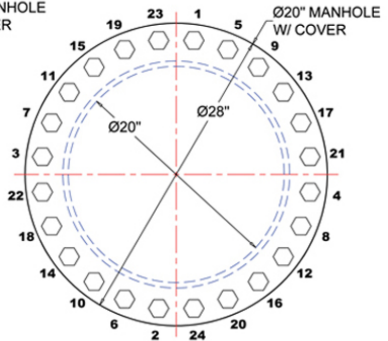
24 BOLT FLANGE not to scale
